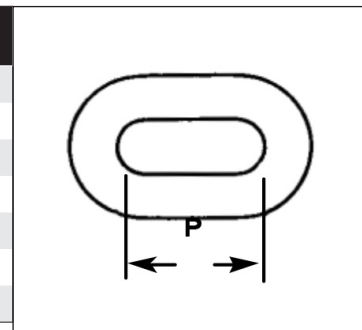
Figure 1 - Chain Wear Measurement
